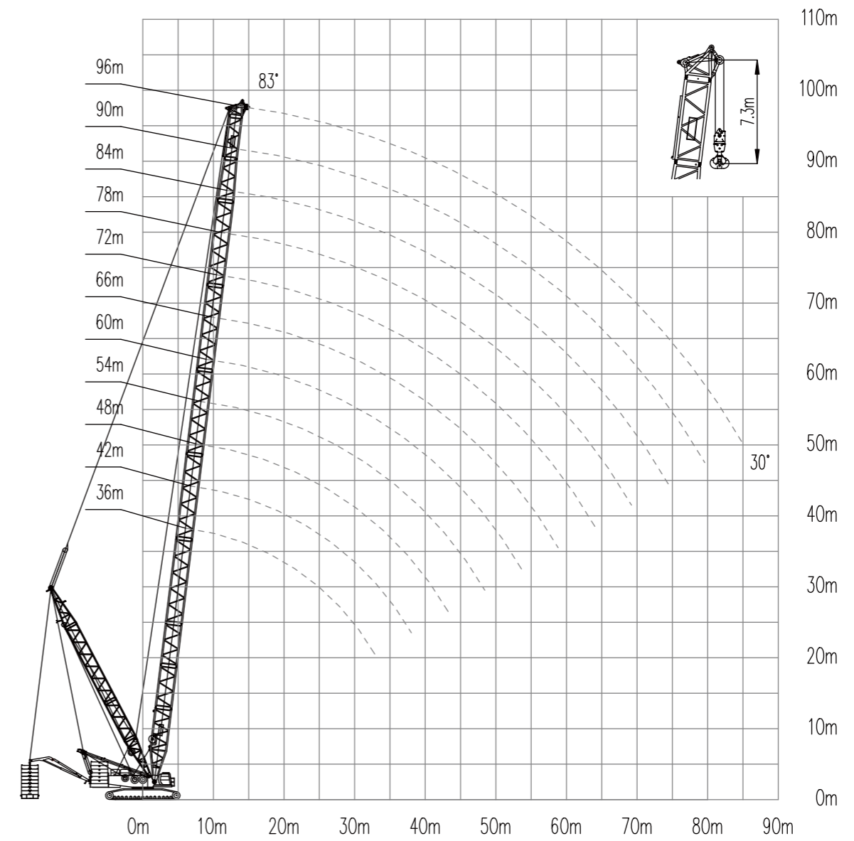
7. Superlift heavy boom working condition (SHB)
