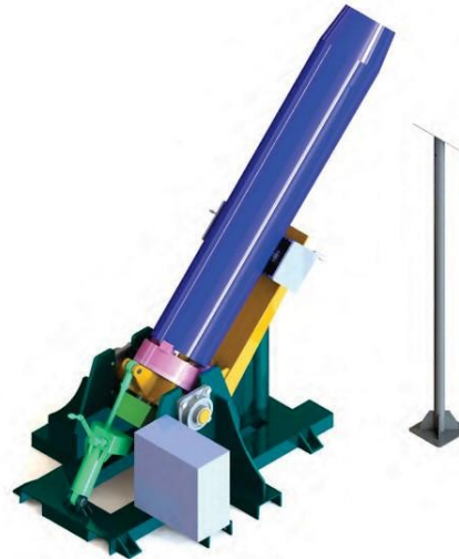
MOTORIZED TILTING WELDING FIXTURE
