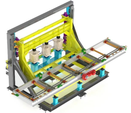
SIDE ARM LIFT TABLE
