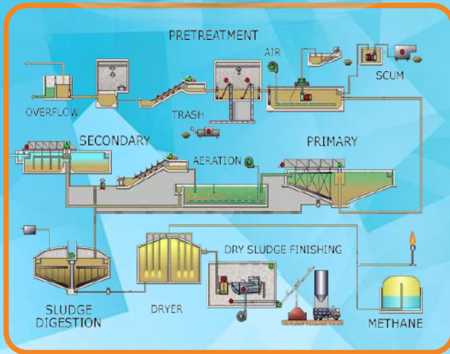
SEWAGE TREATMENT PROCESS
